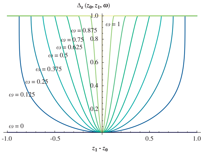
Fig. 3. Graphs of the \Delta z -function for different values of \omega .
