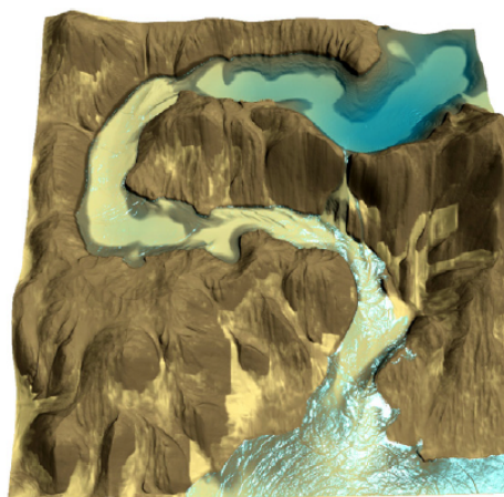
Figure 3: The eroded terrain is obtained by simulating the movement of the water flow and transportation of rock particles [SBBK08].
