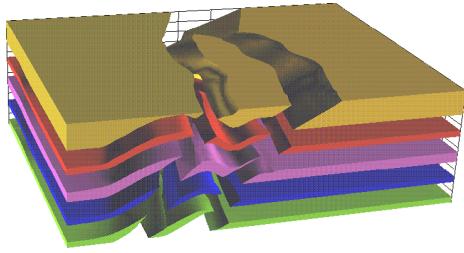
Figure 11: The work by Euler et al. [ESD98] presents a solid model made from the surfaces in the Standard overthrust SEG-EAEG 1994 model [ABN*94].
